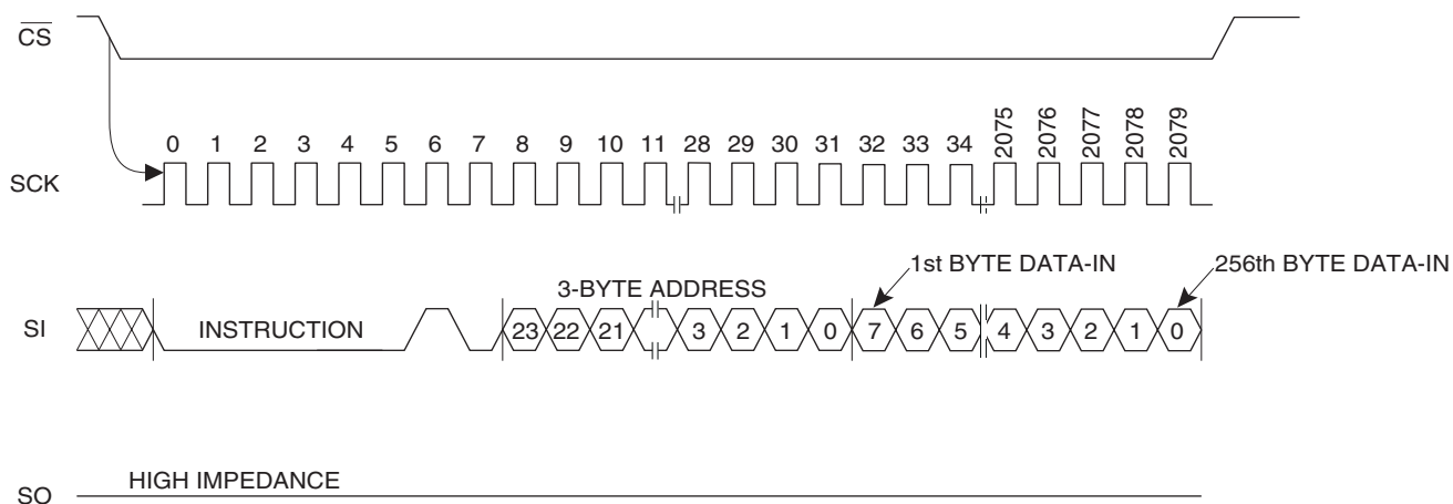
Figure 3-7. PROGRAM Timing
